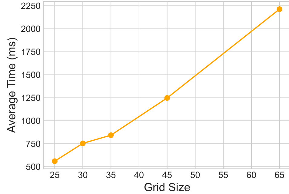
Performance Scaling by Grid Size
